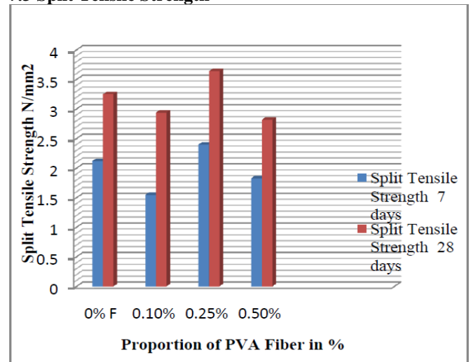
Fig.11: Split Tensile Strength of Polyvinyl alcohol Fiber after 7th and 28th days
