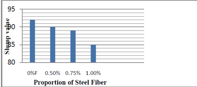
Fig.8: Slump Value of Fresh Concretes for Polyvinyl alcohol Fiber
