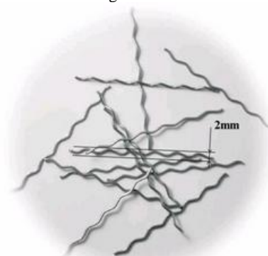
Fig. 1: Steel Fibre – Crimped
