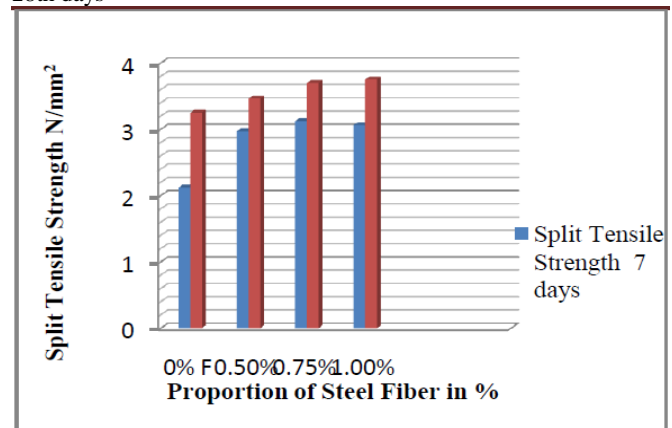
Fig.12: Split Tensile Strength of Steel Fiber after 7th and 28th days Inference
