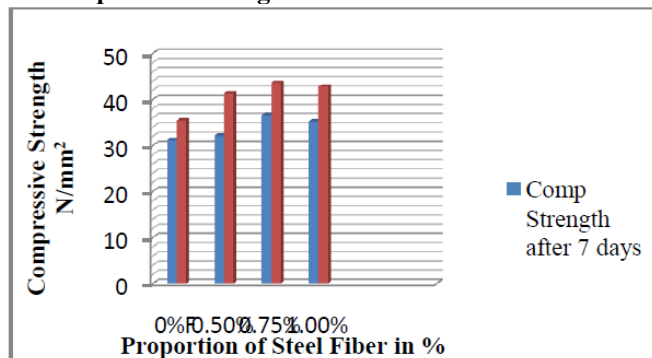
Fig.9: Compressive Strength of Steel Fiber after 7th and 28th days Inference
