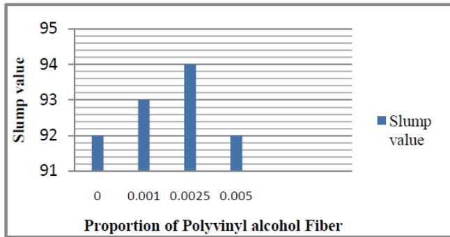
Fig.7: Slump Value of Fresh Concretes for Polyvinyl alcohol Fiber
