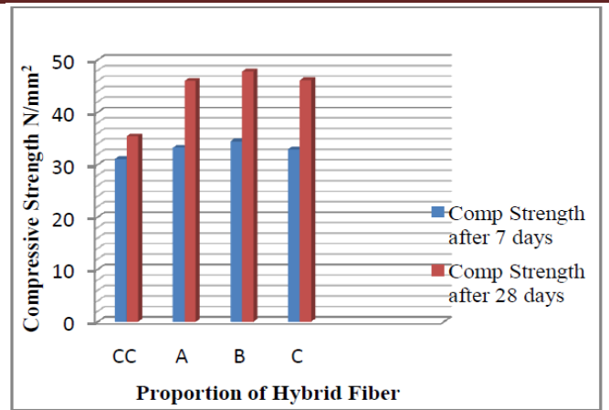
Fig.10: Compressive strength of Hybrid fiber after 7th and 28th days 7.2.1 Inference
